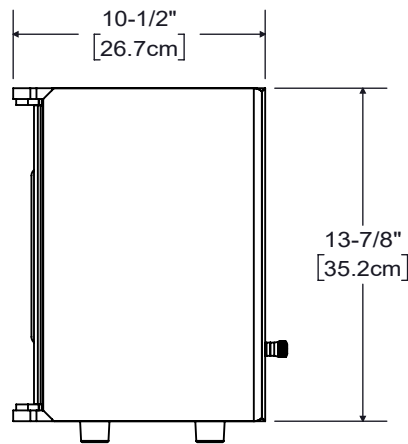
Right view
